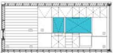
LONG SECTION 01
